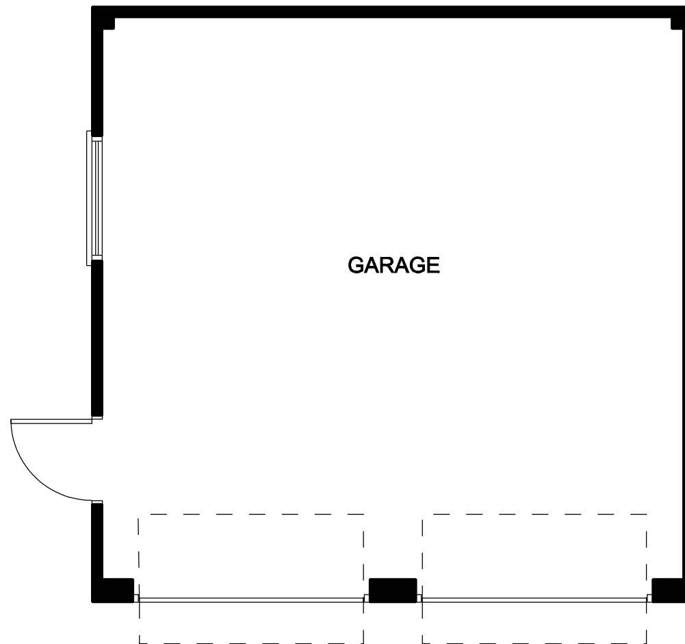
GARAGE PLAN (GARAGE AT REAR OF FLAT)
